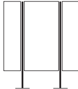
central: 599 x 1,199 x 55 mm wings: 299 x 1,199 x 55 mm
