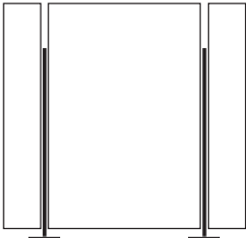
central: 1,199 x 1,799 x 55 mm wings: 299 x 1,799 x 55 mm
